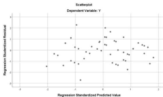
Gambar 1. Hasil scatterplot
